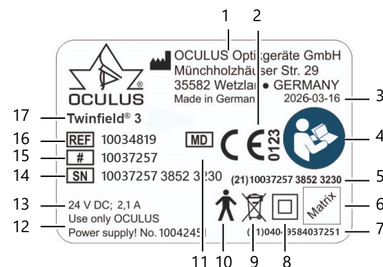
Fig. 2-1: Type plate (example)
