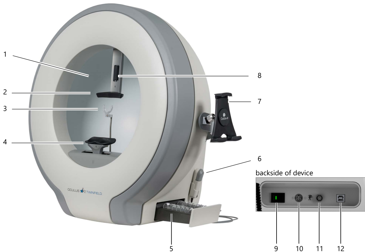
Fig. 3-1: Parts of the device
