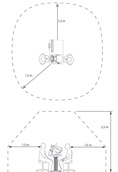
Fig. 4-1: Patient environment (for example, with Smartfield)
