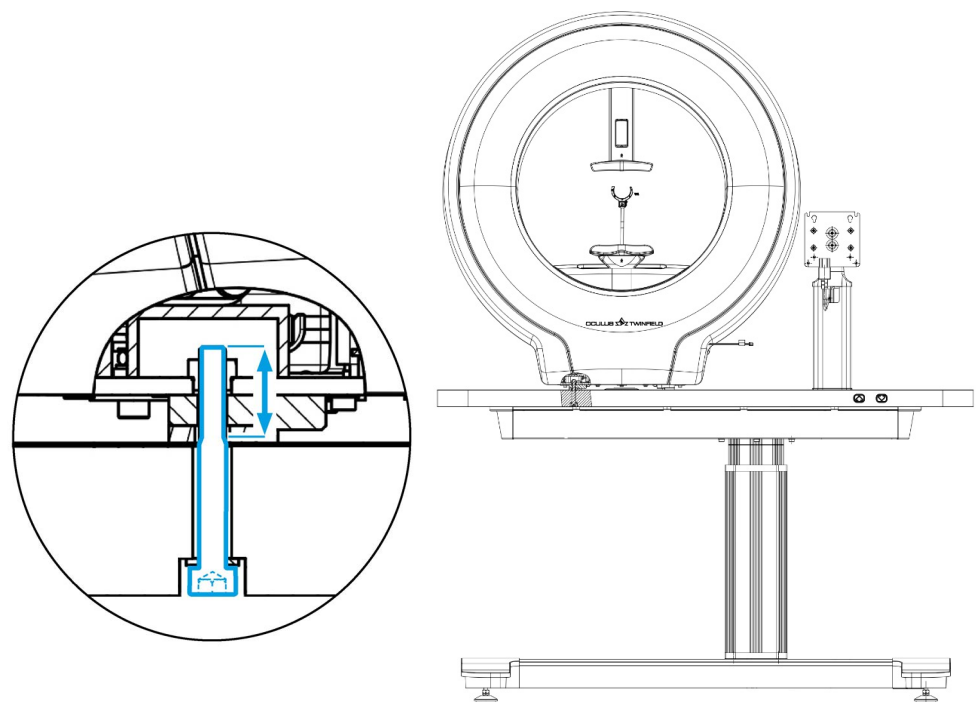
Fig. 4-2: Maximum screw protrusion above the top edge of the ophthalmic table, lift column, etc.
