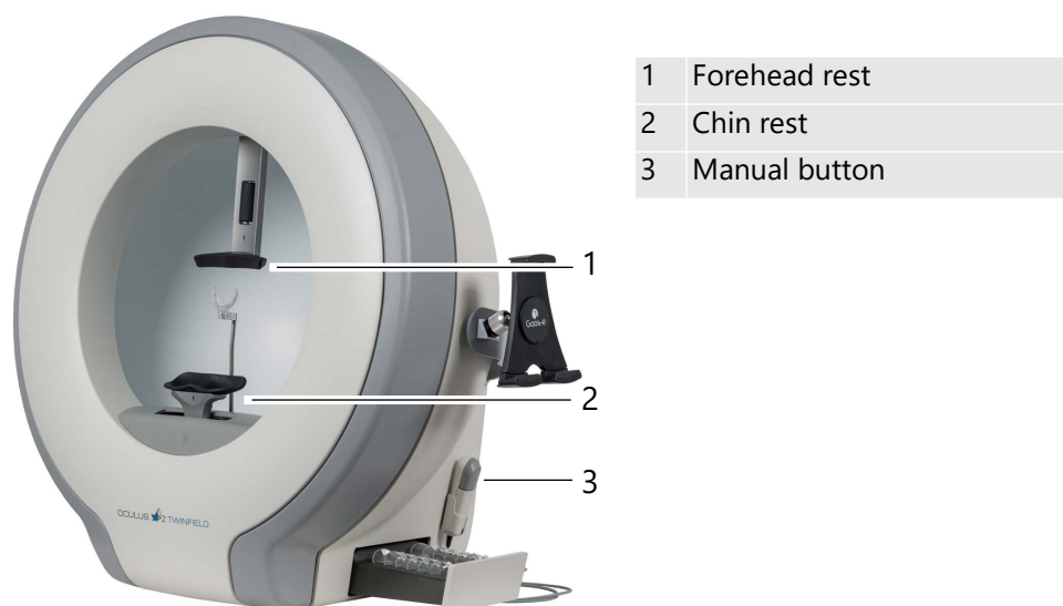
Fig. 3-3: Application parts
